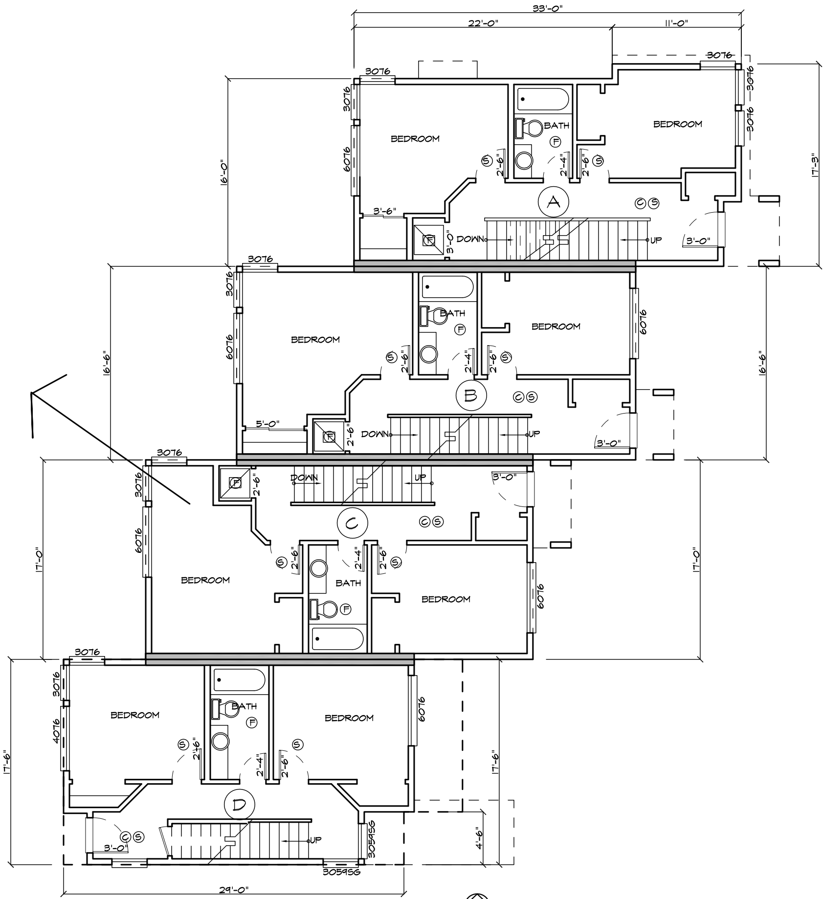
FIRST FLOOR PLAN BUILDING 1
