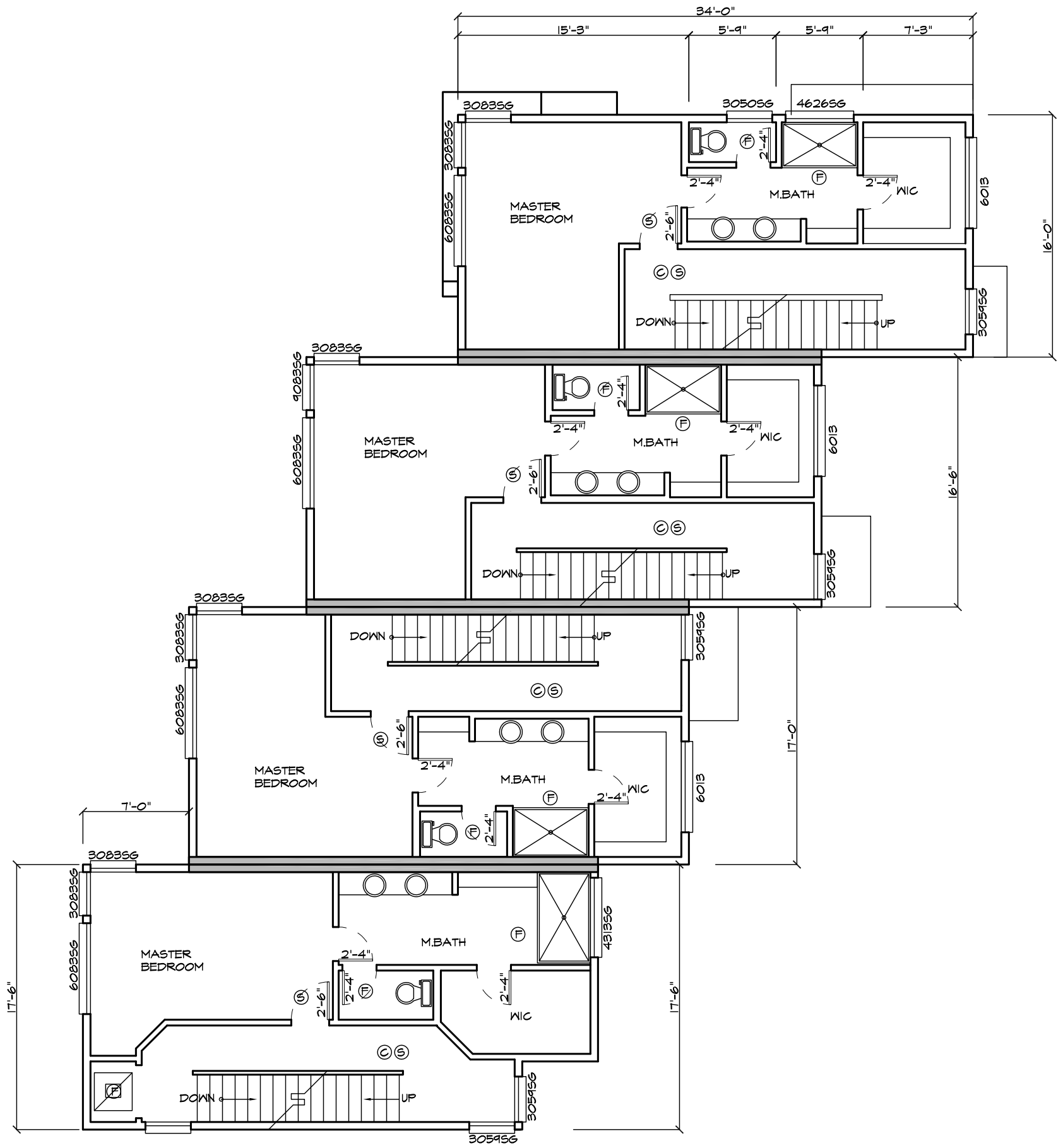
THIRD FLOOR PLAN BUILDING I
