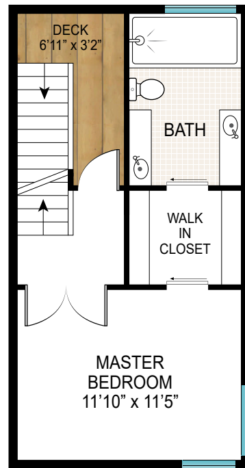
THIRD FLOOR
